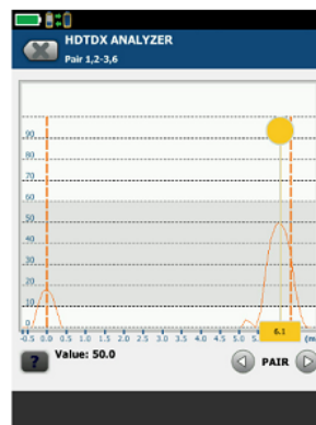
High Definition Time Domain Cross talk (HDTX) shows the far end connection is clearly the issue
